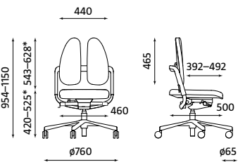
XENIUM OPERATIVE DUO-BACK ESP-ST Weight | Waga 16.20 kg
