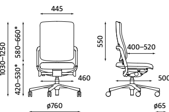
XENIUM OPERATIVE UPH IND-ST Weight | Waga 16.00 kg
