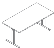
PSU07 1390 / 695 / 725 25 kg
