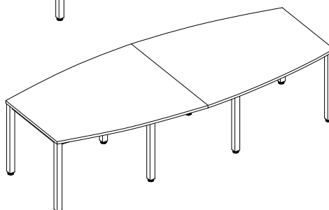
2400, 2800 × 1200/800 × 740 mm, 3200, 3600, 4000 × 1400/1000 × 740 mm
